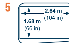
Aft lower deck cargo door (STA 1865) Right-hand side
